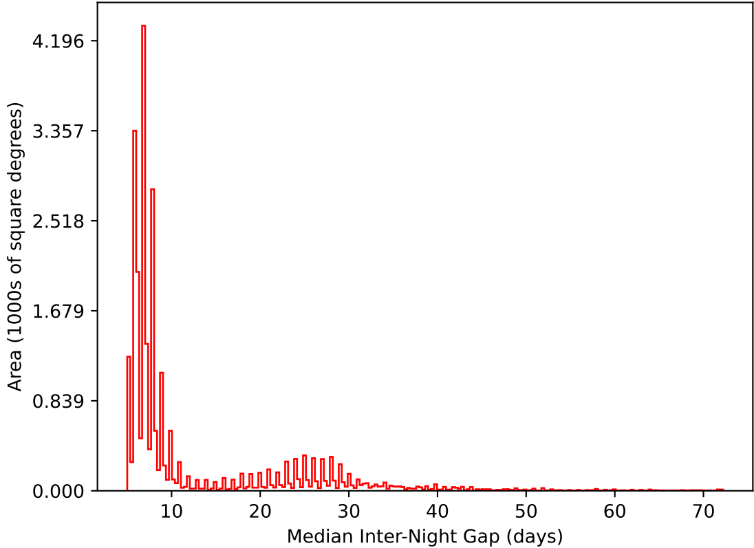
ddf_acor_sf30_lsf40_lsr10_v3.4_10yrs All sky i band: Median Inter-Night Gap
