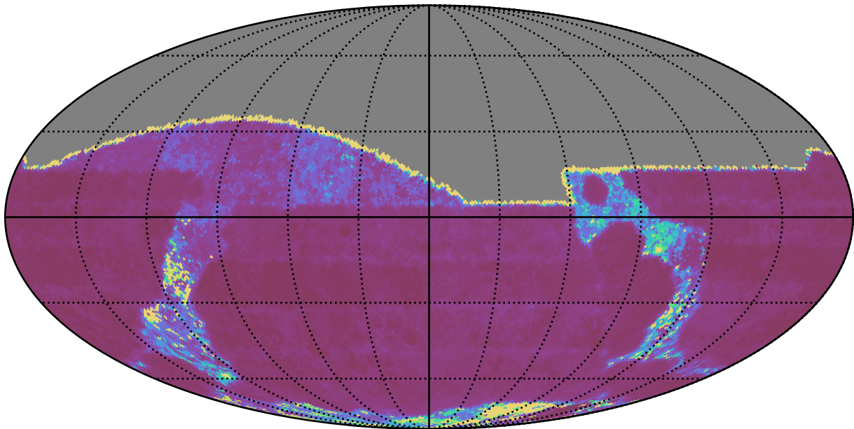
ddf_acor_sf30_lsf40_lsr10_v3.4_10yrs All sky g band: Median Inter-Night Gap
