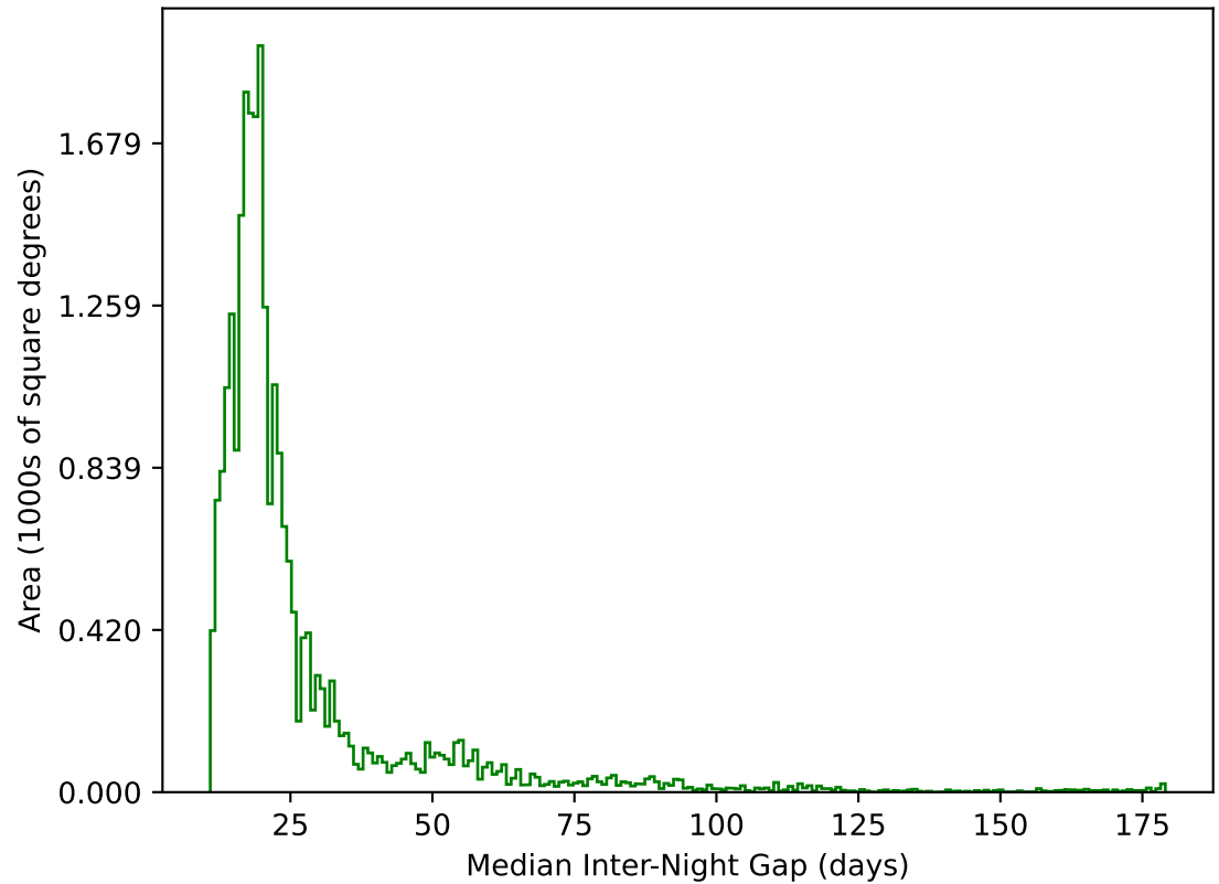
ddf_acor_sf30_lsf40_lsr10_v3.4_10yrs All sky g band: Median Inter-Night Gap
