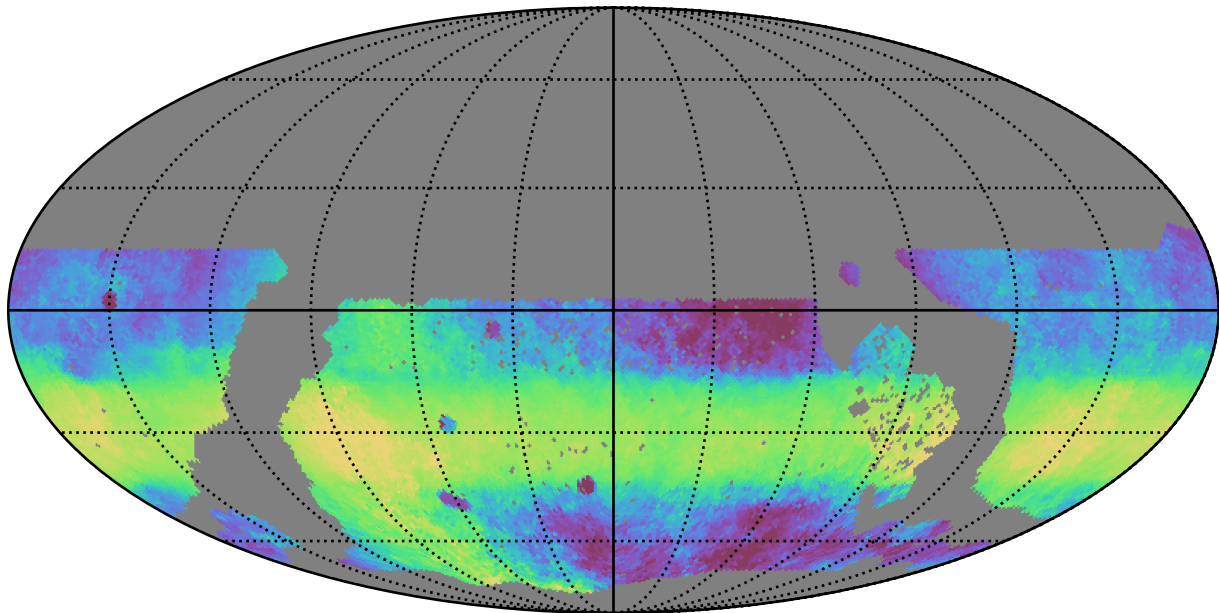
ddf_acor_sf30_lsf40_lsr10_v3.4_10yrs WFD y band: Median HA
