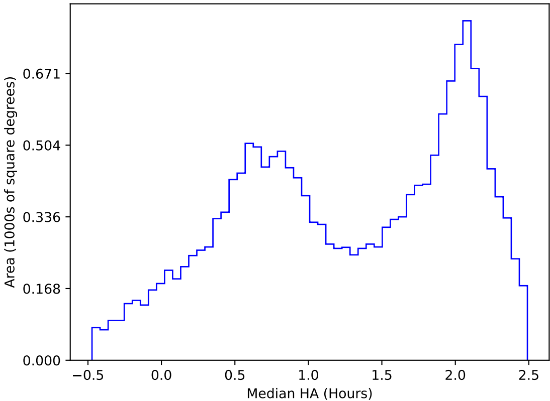
ddf_acor_sf30_lsf40_lsr10_v3.4_10yrs WFD y band: Median HA
