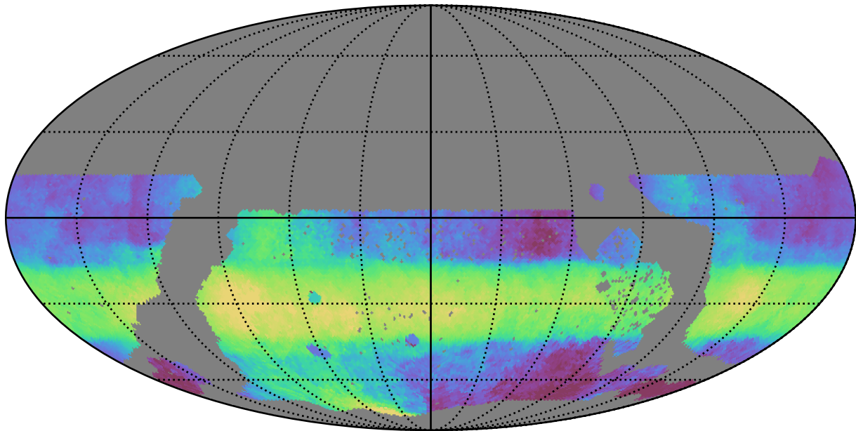
ddf_acor_sf30_lsf40_lsr10_v3.4_10yrs WFD r band: Median HA
