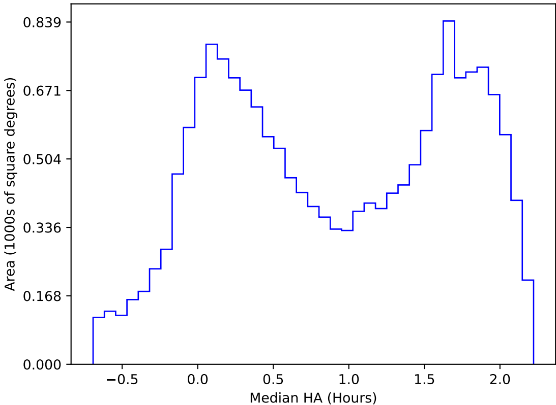
ddf_acor_sf30_lsf40_lsr10_v3.4_10yrs WFD r band: Median HA
