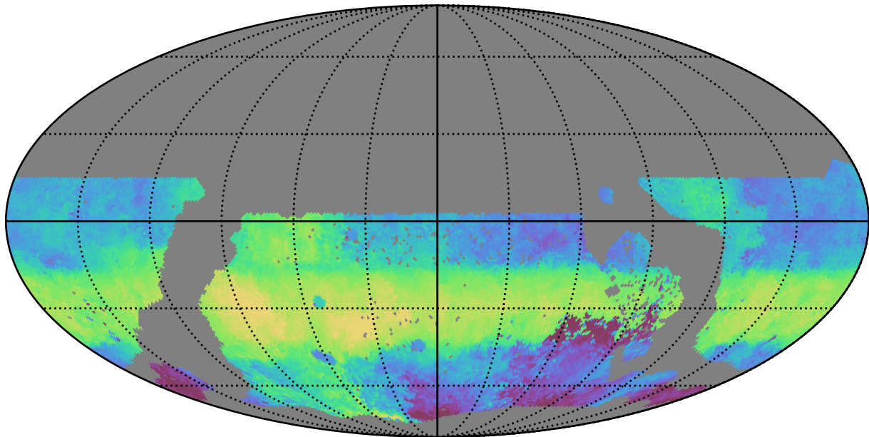
ddf_acor_sf30_lsf40_lsr10_v3.4_10yrs WFD g band: Median HA
