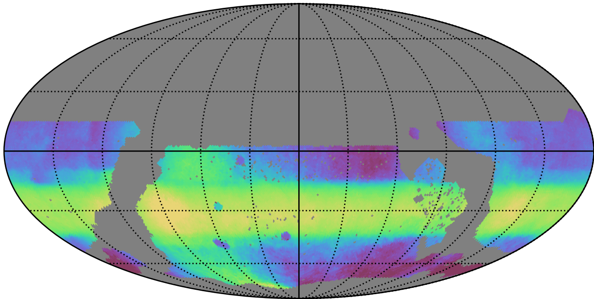
ddf_acor_sf30_lsf40_lsr10_v3.4_10yrs WFD all bands: Median HA
