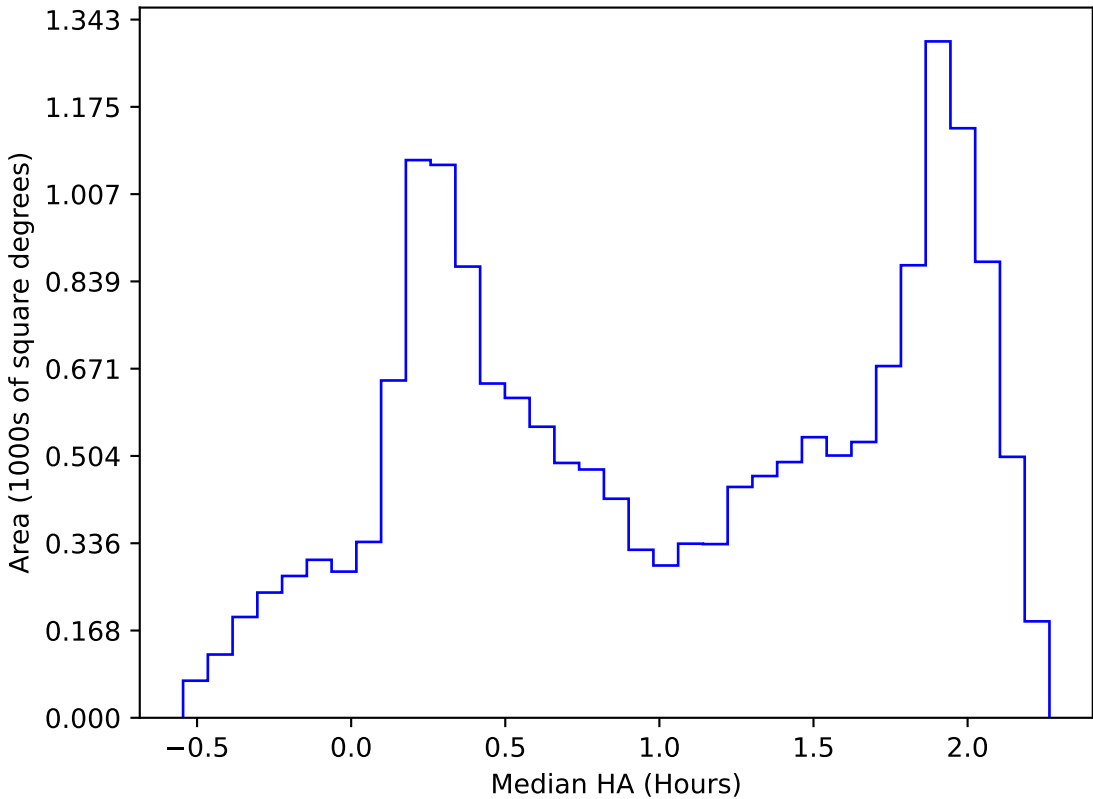
ddf_acor_sf30_lsf40_lsr10_v3.4_10yrs WFD all bands: Median HA
