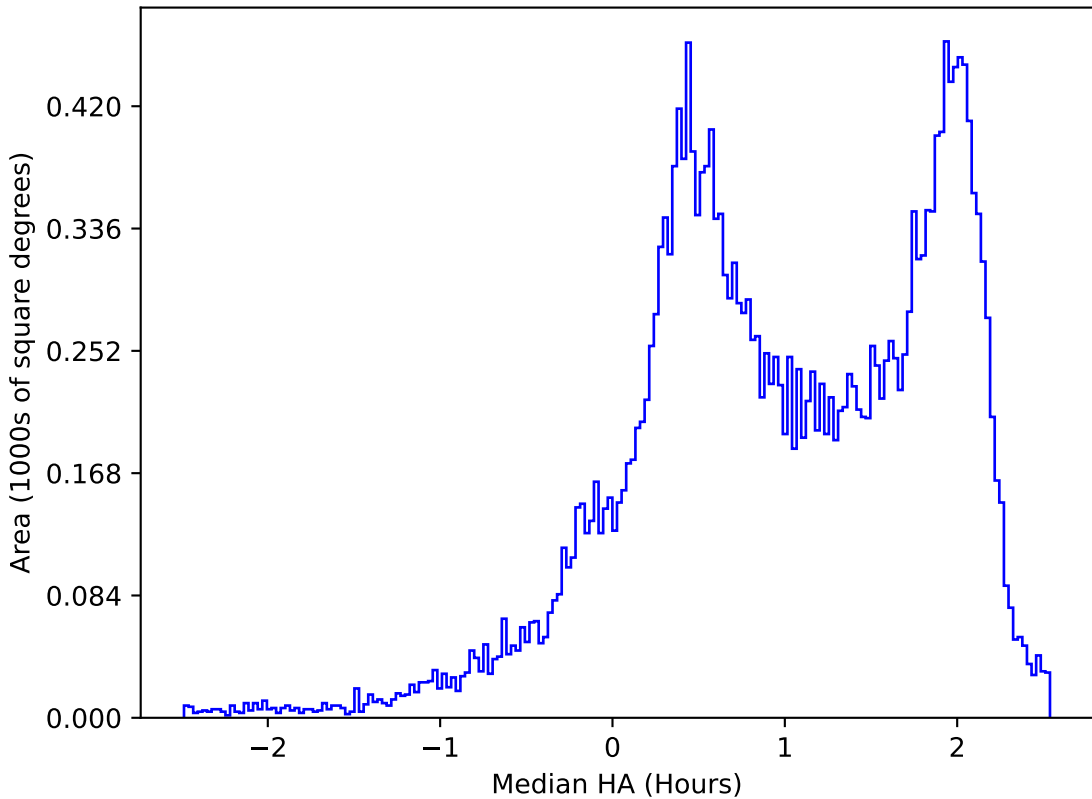
ddf_acor_sf30_lsf40_lsr10_v3.4_10yrs All sky z band: Median HA
