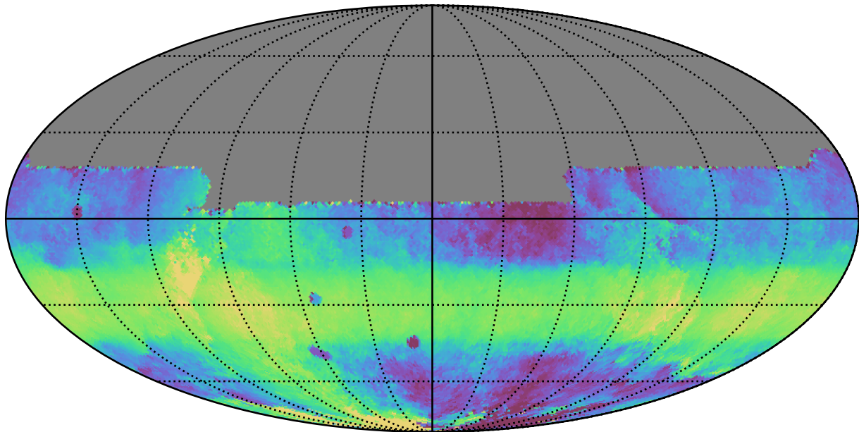
ddf_acor_sf30_lsf40_lsr10_v3.4_10yrs All sky y band: Median HA
