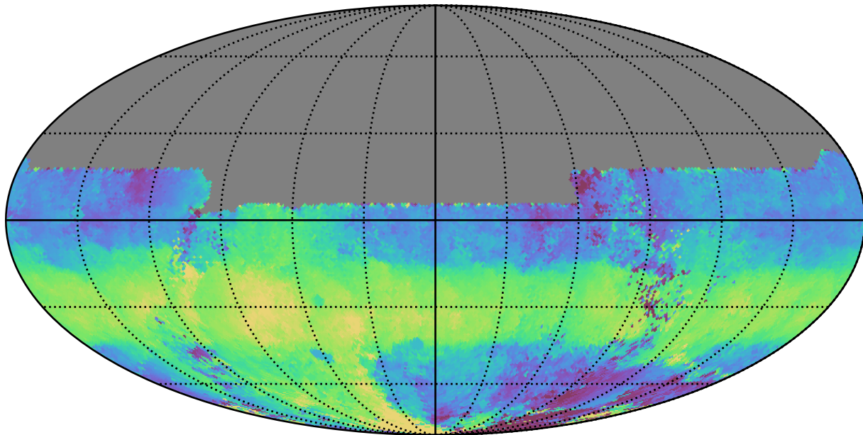
ddf_acor_sf30_lsf40_lsr10_v3.4_10yrs All sky u band: Median HA
