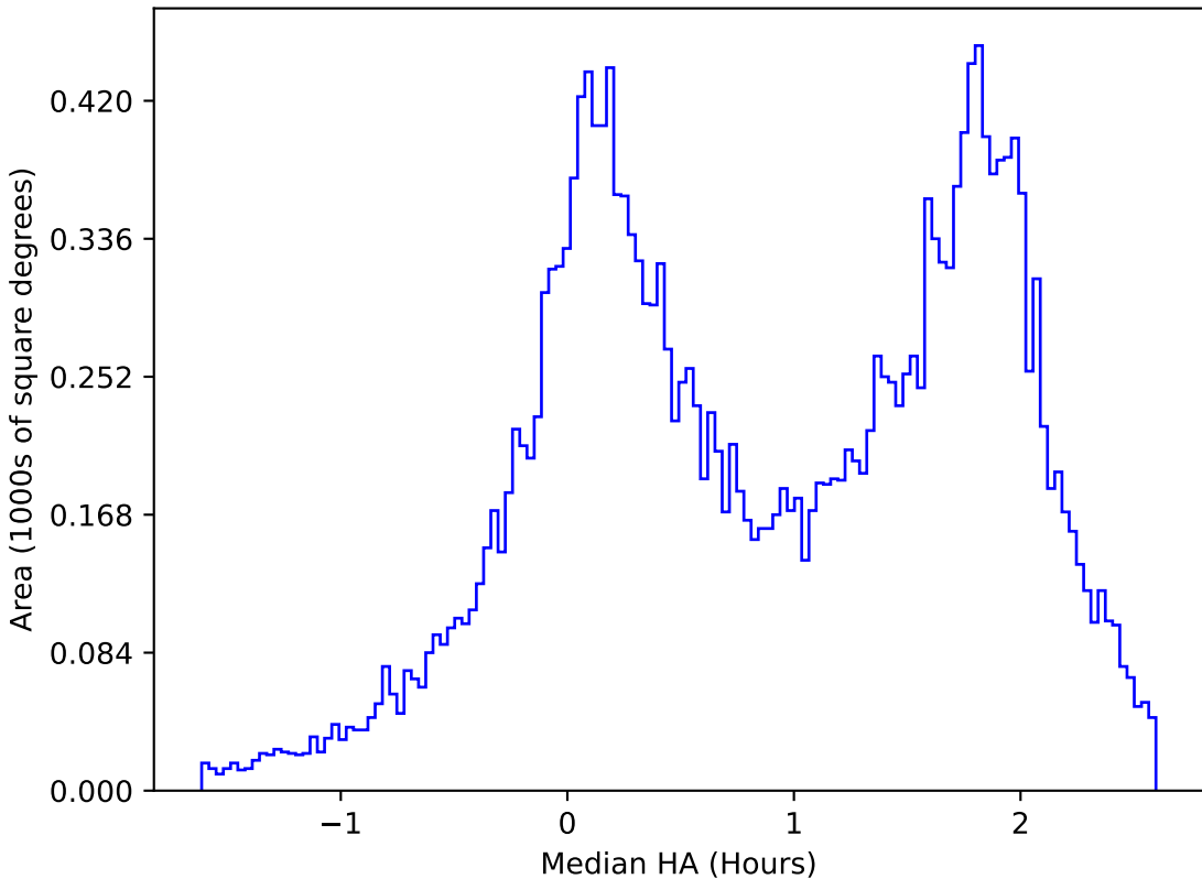
ddf_acor_sf30_ls40_lsr10_v3.4_10yrs All sky u band: Median HA
