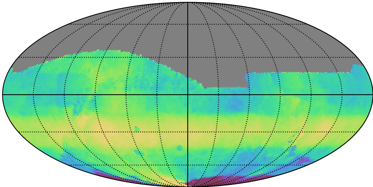
ddf_acor_sf30_lsf40_lsr10_v3.4_10yrs All sky r band: Median HA
