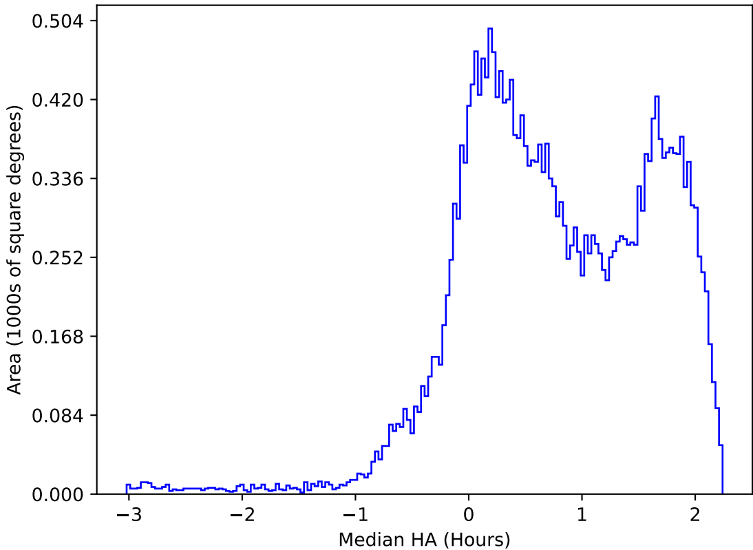
ddf_acor_sf30_lsf40_lsr10_v3.4_10yrs All sky r band: Median HA
