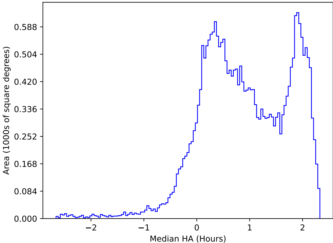
ddf_acor_sf30_lsf40_lsr10_v3.4_10yrs All sky i band: Median HA
