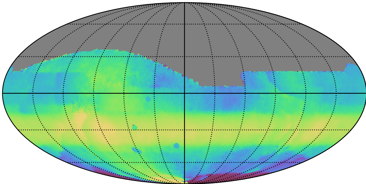
ddf_acor_sf30_lsf40_lsr10_v3.4_10yrs All sky all bands: Median HA
