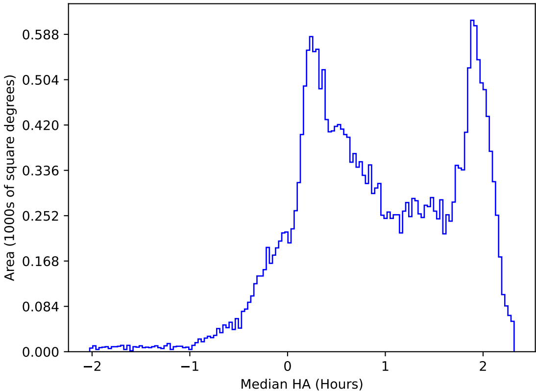
ddf_acor_sf30_lsf40_lsr10_v3.4_10yrs All sky all bands: Median HA
