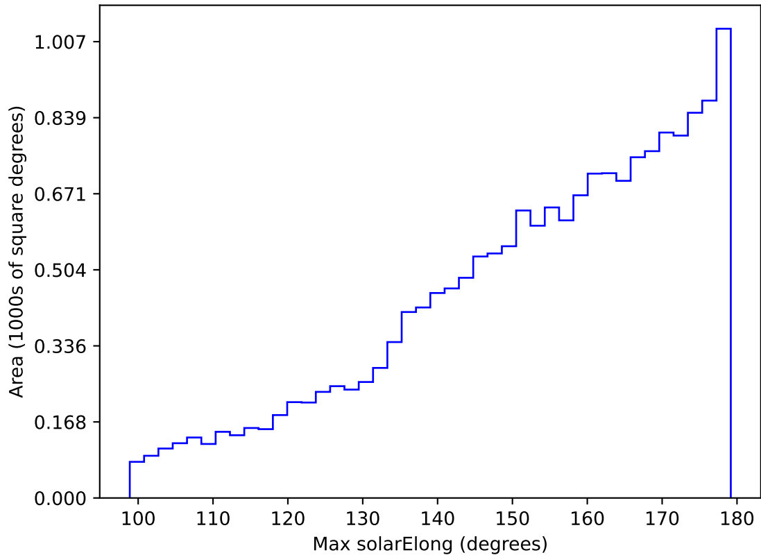
ddf_acor_sf30_lsf40_lsr10_v3.4_10yrs WFD y band: Max solarElong
