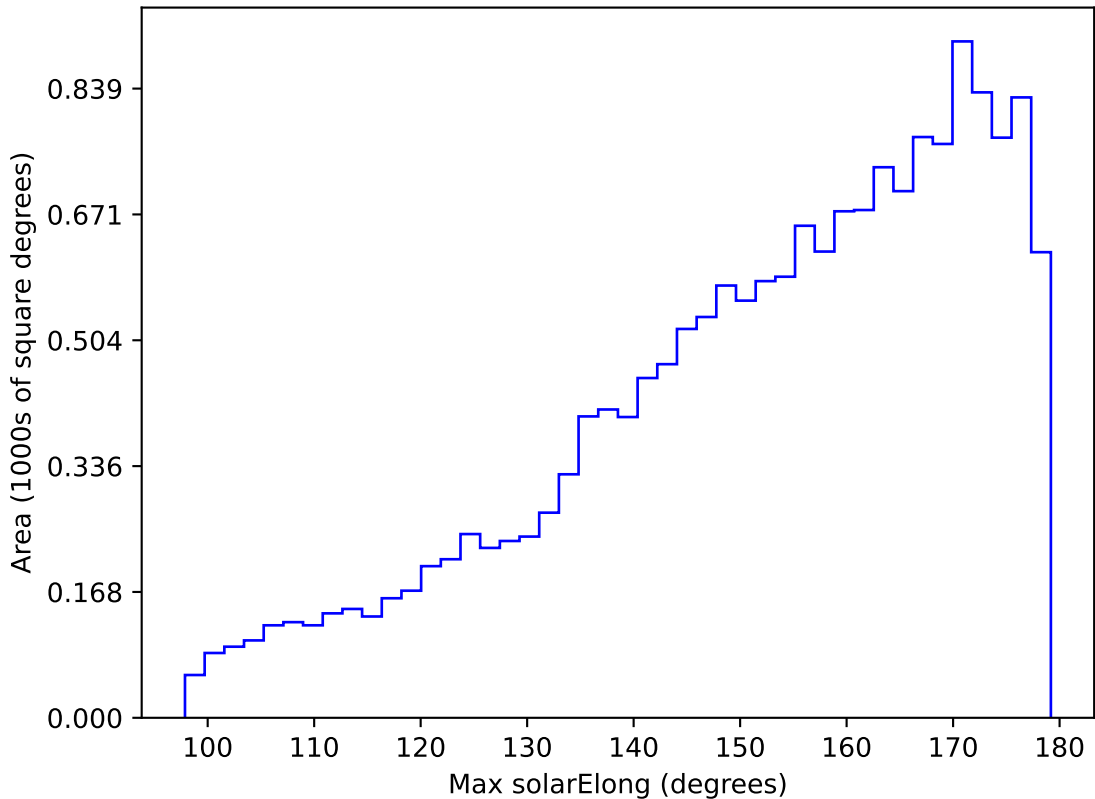
ddf_acor_sf30_lsf40_lsr10_v3.4_10yrs WFD u band: Max solarElong
