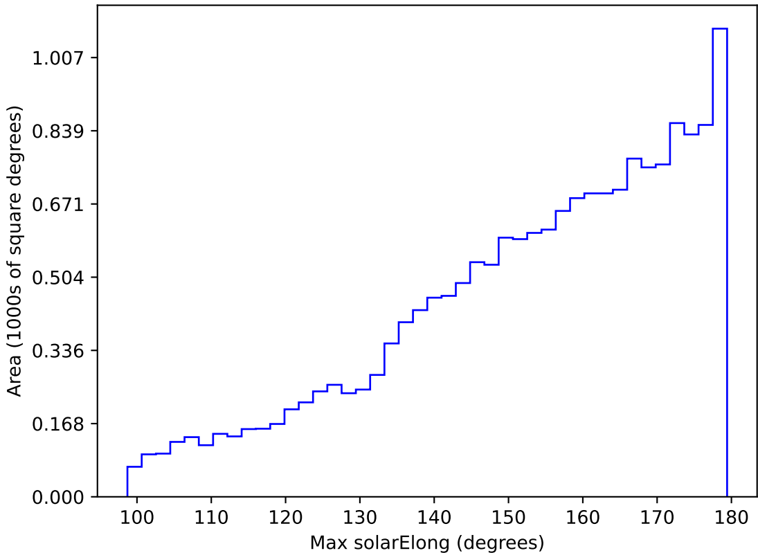
ddf_acor_sf30_lsf40_lsr10_v3.4_10yrs WFD r band: Max solarElong
