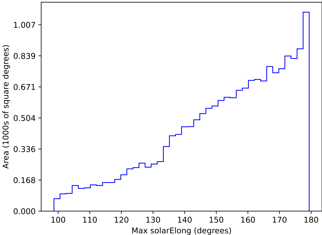
ddf_acor_sf30_lsf40_lsr10_v3.4_10yrs WFD i band: Max solarElong
