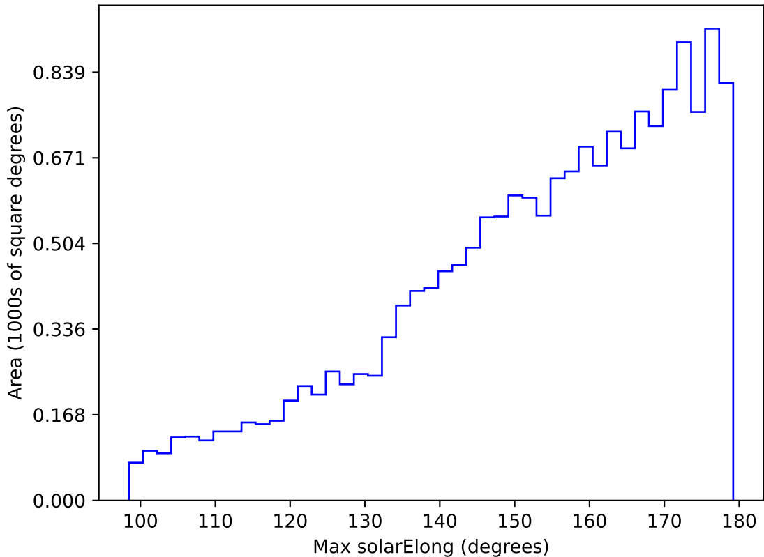
ddf_acor_sf30_lsf40_lsr10_v3.4_10yrs WFD g band: Max solarElong
