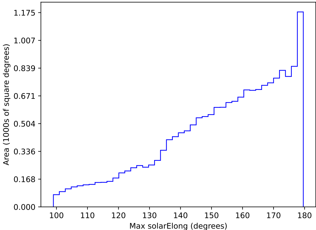
ddf_acor_sf30_lsf40_lsr10_v3.4_10yrs WFD all bands: Max solarElong
