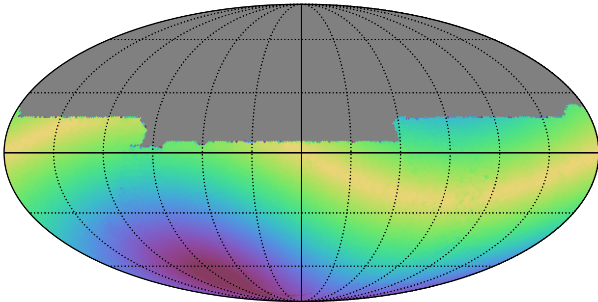
ddf_acor_sf30_lsf40_lsr10_v3.4_10yrs All sky y band: Max solarElong
