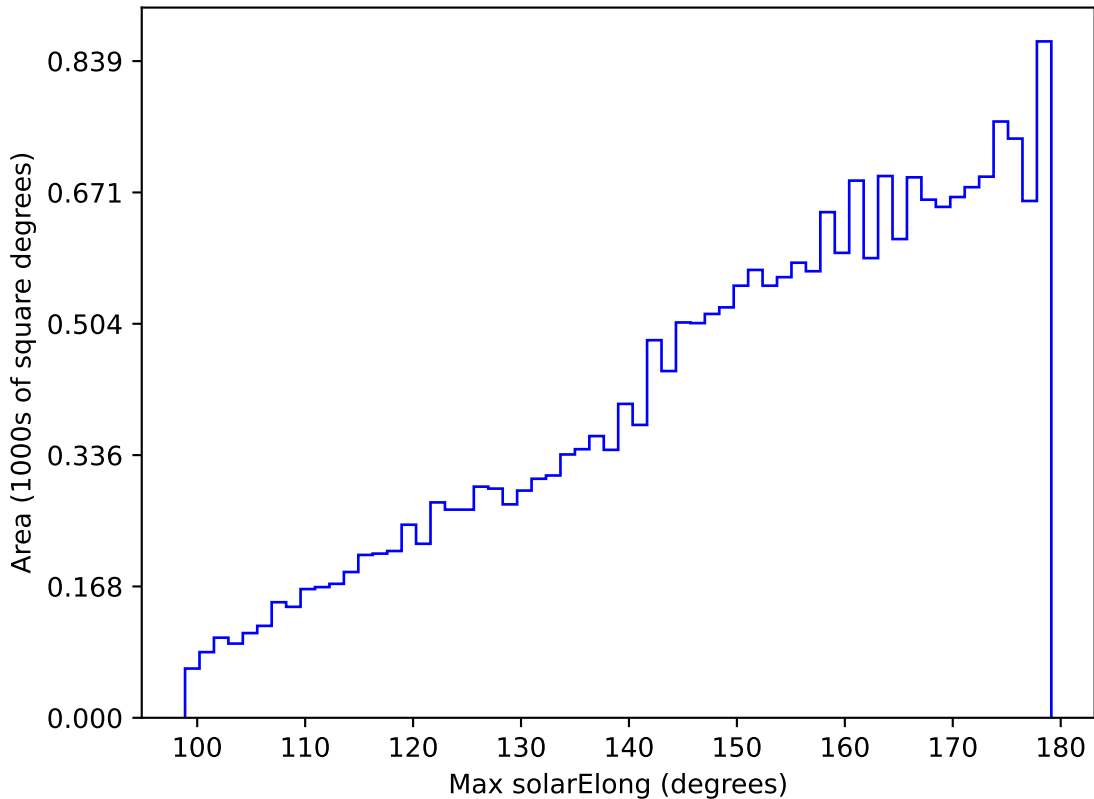
ddf_acor_sf30_lsf40_lsr10_v3.4_10yrs All sky y band: Max solarElong
