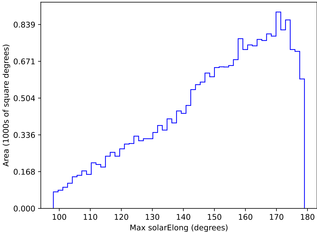
ddf_acor_sf30_lsf40_lsr10_v3.4_10yrs All sky u band: Max solarElong
