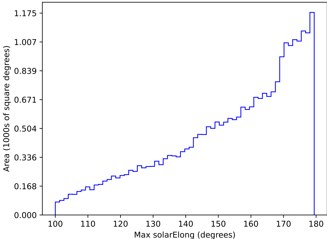
ddf_acor_sf30_lsf40_lsr10_v3.4_10yrs All sky r band: Max solarElong
