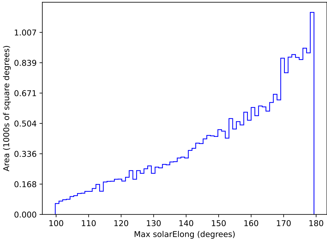
ddf_acor_sf30_lsf40_lsr10_v3.4_10yrs All sky i band: Max solarElong
