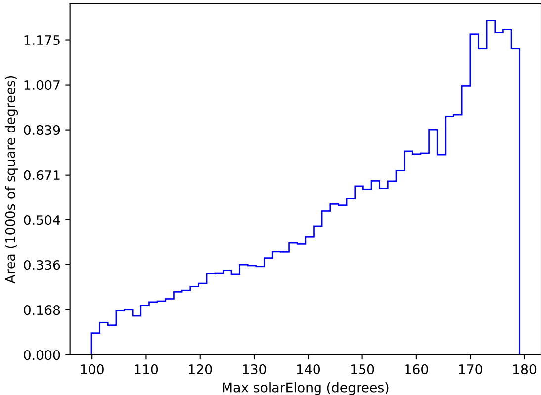
ddf_acor_sf30_lsf40_lsr10_v3.4_10yrs All sky g band: Max solarElong
