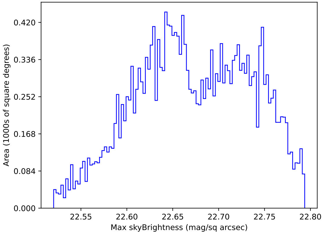
ddf_acor_sf30_lsf40_lsr10_v3.4_10yrs Yr 1 u band: Max skyBrightness
