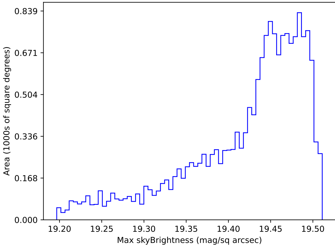
ddf_acor_sf30_lsf40_lsr10_v3.4_10yrs WFD z band: Max skyBrightness
