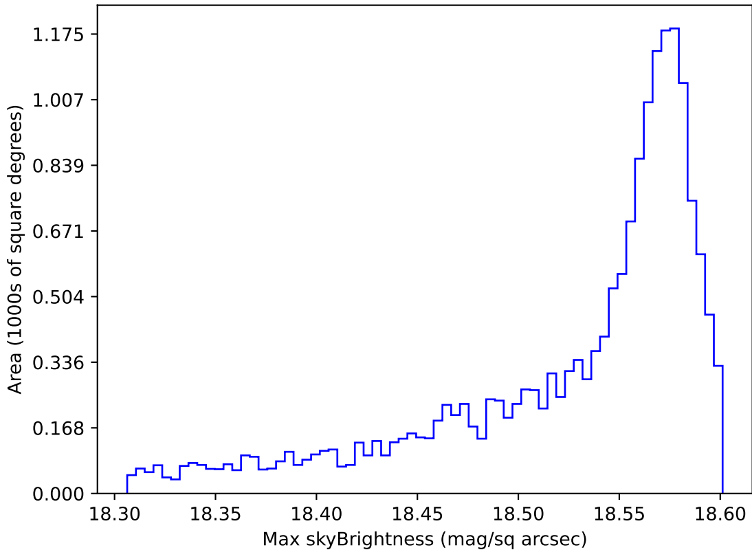
ddf_acor_sf30_lsf40_lsr10_v3.4_10yrs WFD y band: Max skyBrightness
