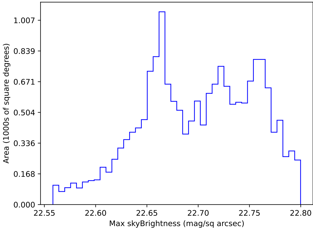
ddf_acor_sf30_lsf40_lsr10_v3.4_10yrs WFD u band: Max skyBrightness
