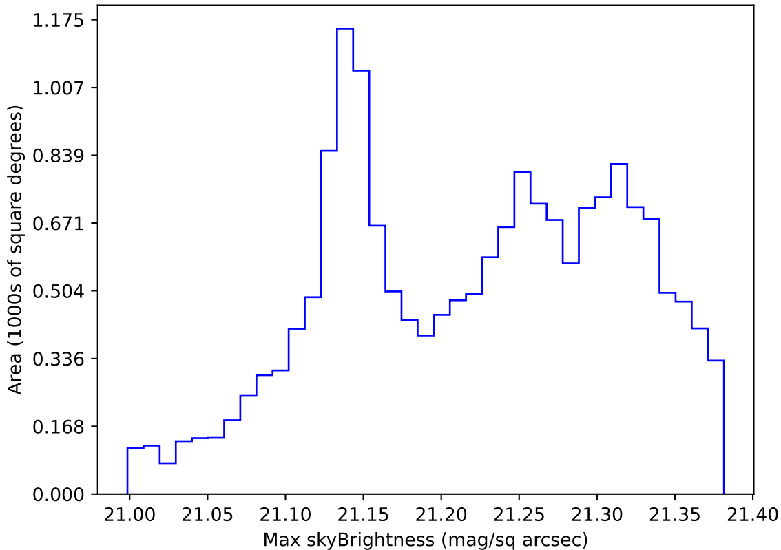
ddf_acor_sf30_lsf40_lsr10_v3.4_10yrs WFD r band: Max skyBrightness
