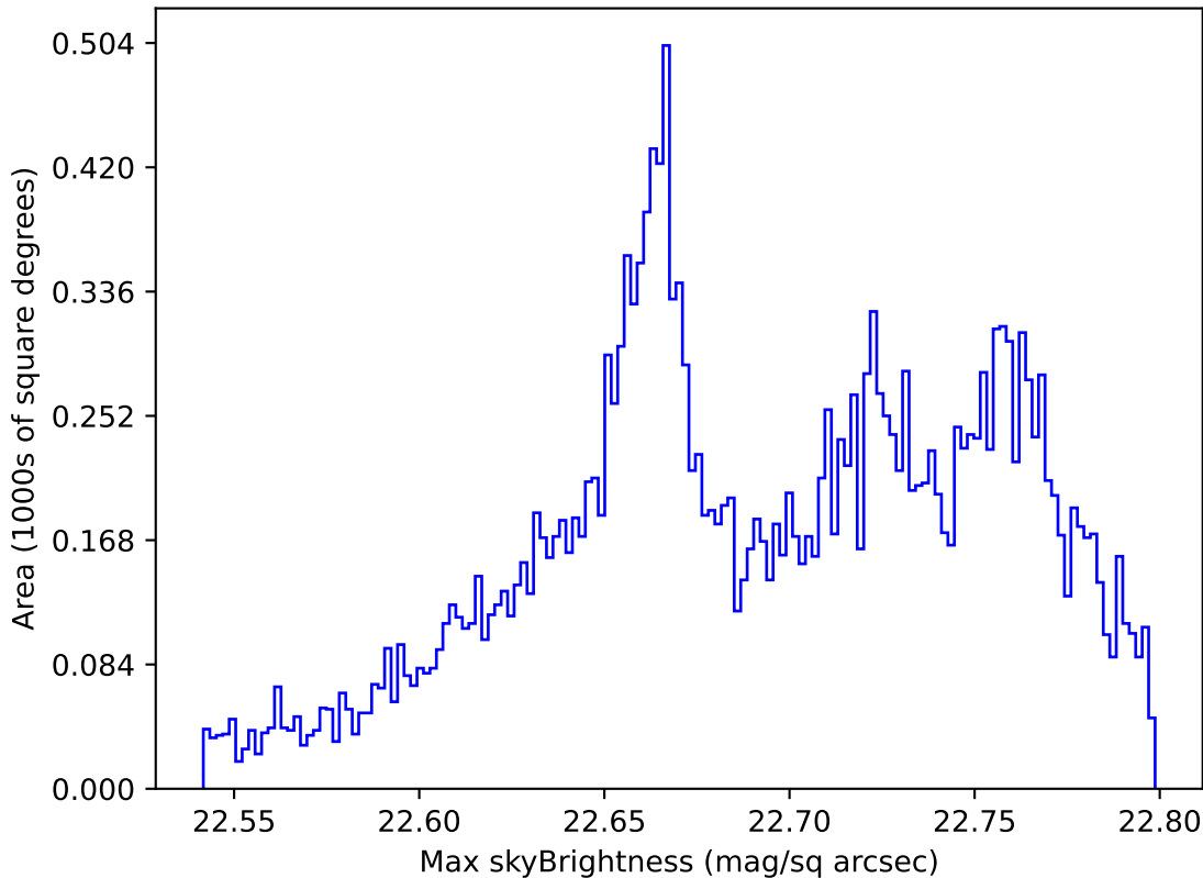
ddf_acor_sf30_lsf40_lsr10_v3.4_10yrs All sky u band: Max skyBrightness
