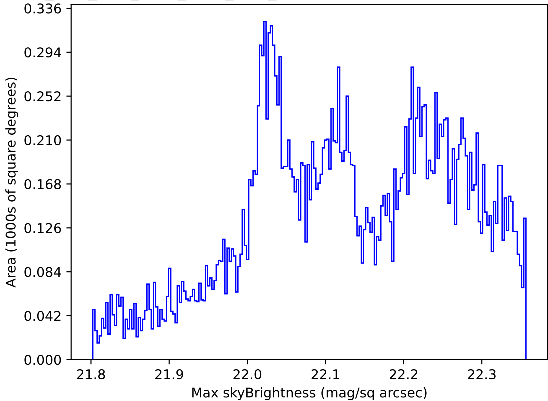
ddf_acor_sf30_lsf40_lsr10_v3.4_10yrs All sky g band: Max skyBrightness
