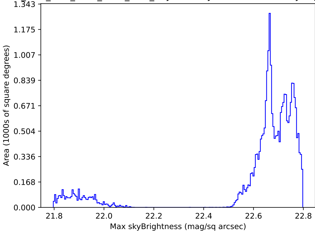
ddf_acor_sf30_lsf40_lsr10_v3.4_10yrs All sky all bands: Max skyBrightness
