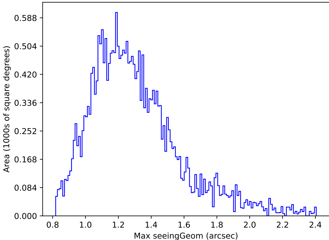
ddf_acor_sf30_lsf40_lsr10_v3.4_10yrs Yr 1 g band: Max seeingGeom
