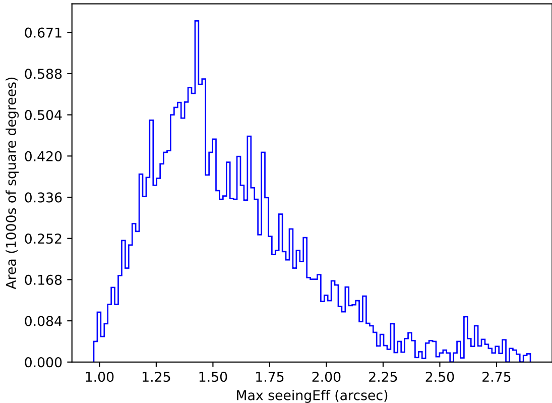
ddf_acor_sf30_lsf40_lsr10_v3.4_10yrs Yr 1 u band: Max seeingEff
