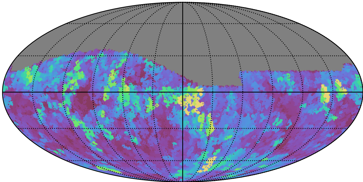
ddf_acor_sf30_lsf40_lsr10_v3.4_10yrs Yr 1 i band: Max seeingEff
