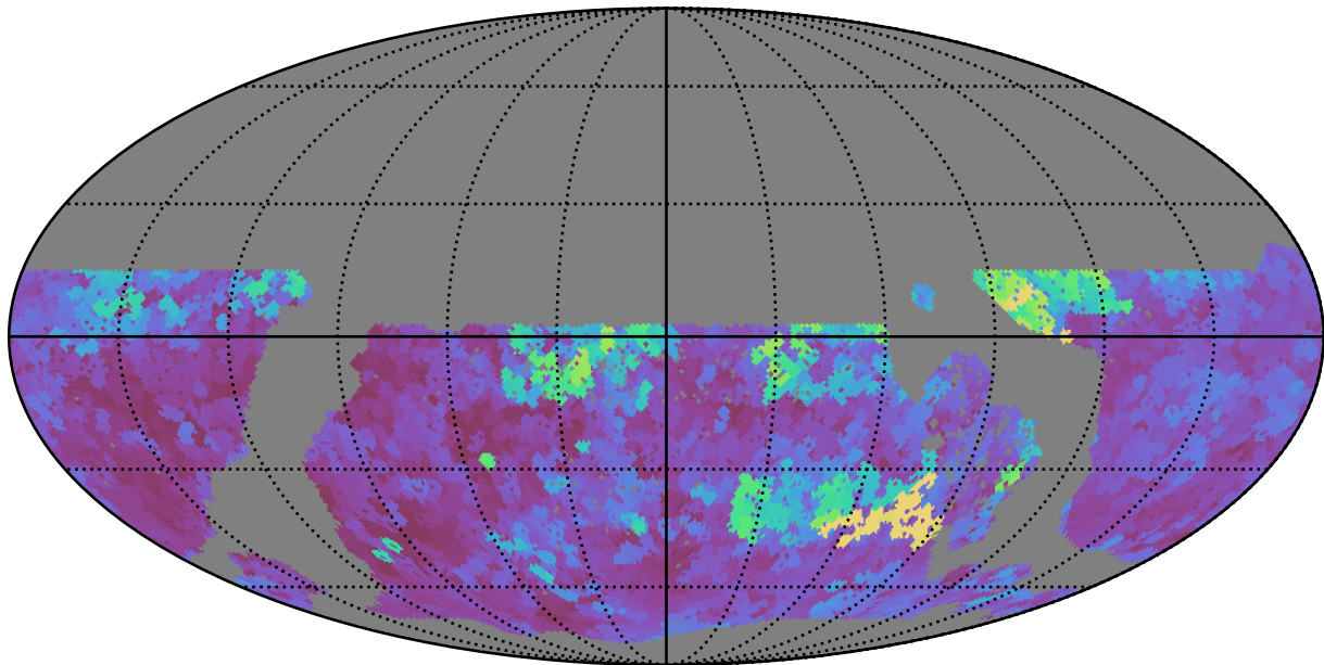
ddf_acor_sf30_lsf40_lsr10_v3.4_10yrs WFD u band: Max seeingEff
