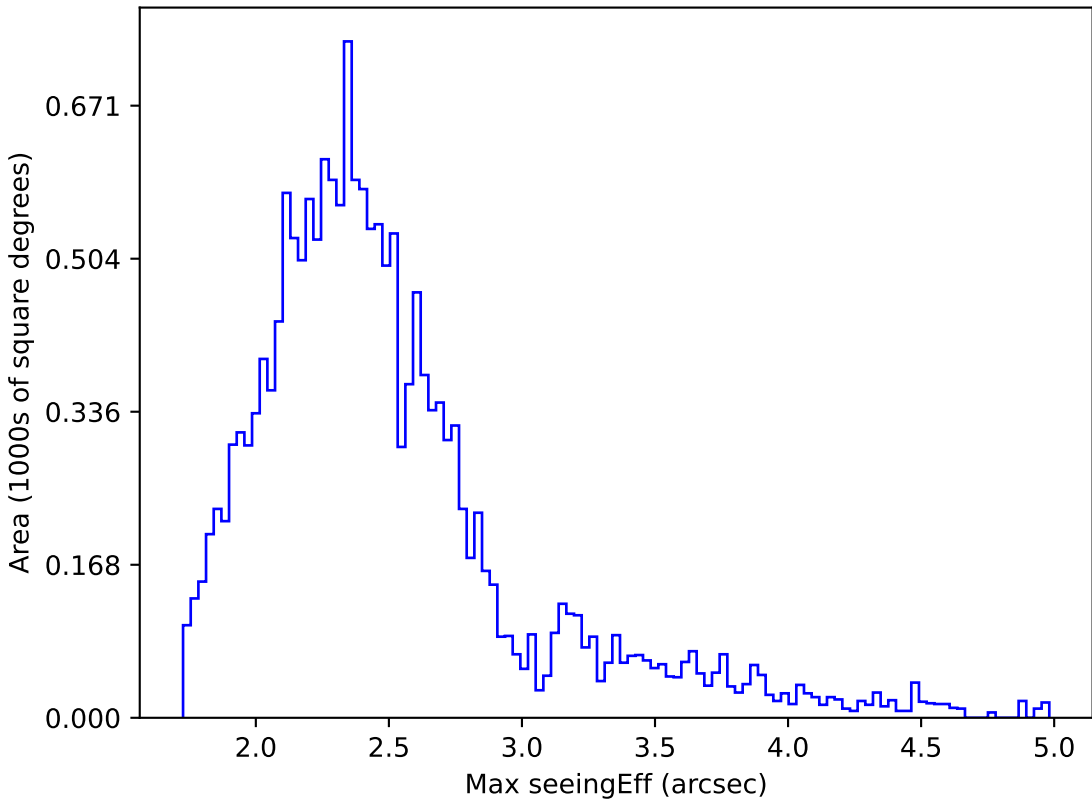
ddf_acor_sf30_lsf40_lsr10_v3.4_10yrs WFD u band: Max seeingEff
