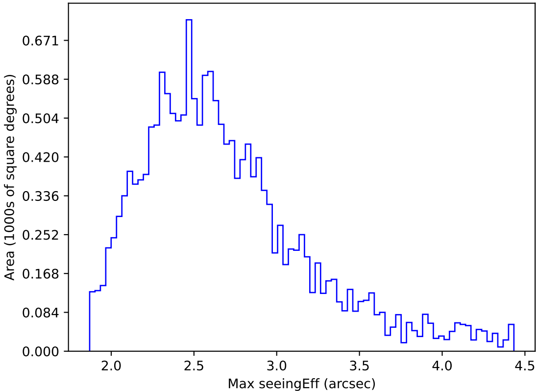
ddf_acor_sf30_Isf40_Isr10_v3.4_10yrs WFD r band: Max seeingEff
