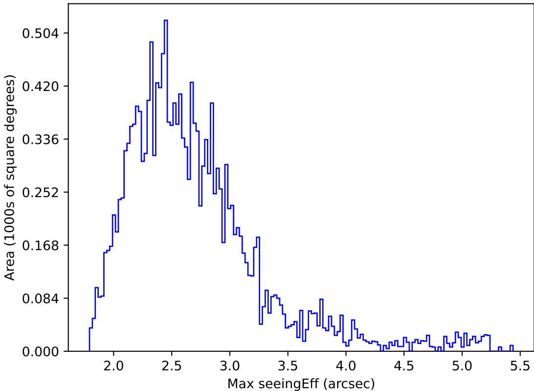
ddf_acor_sf30_lsf40_lsr10_v3.4_10yrs WFD i band: Max seeingEff
