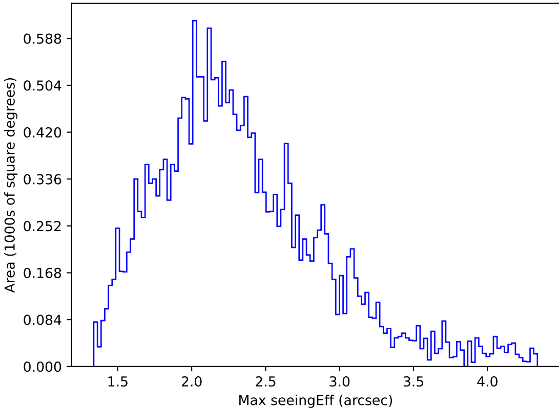
ddf_acor_sf30_ls40_lsr10_v3.4_10yrs All sky y band: Max seeingEff
