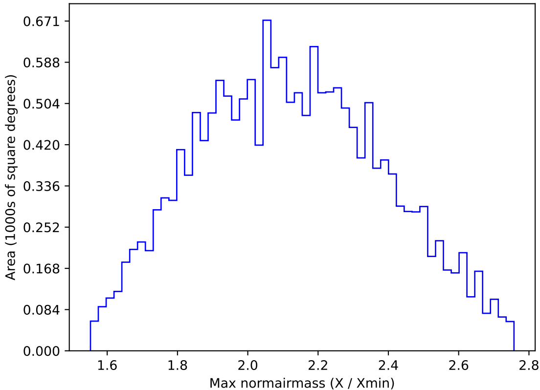
ddf_acor_sf30_lsf40_lsr10_v3.4_10yrs WFD y band: Max normairmass
