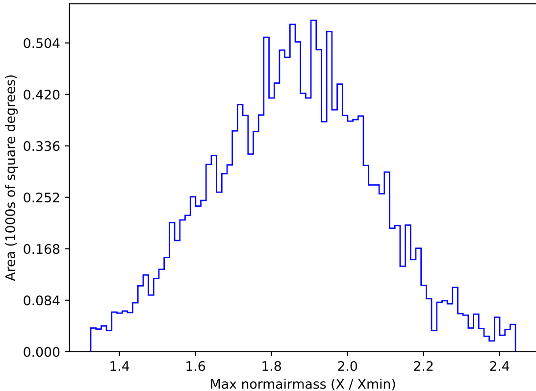
ddf_acor_sf30_lsf40_lsr10_v3.4_10yrs WFD g band: Max normairmass
