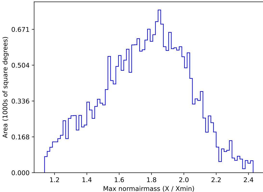
ddf_acor_sf30_lsf40_lsr10_v3.4_10yrs All sky g band: Max normairmass
